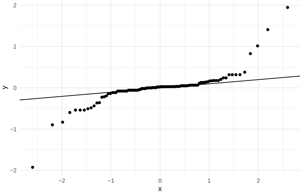
QQ-plot of residuals for NANO model
